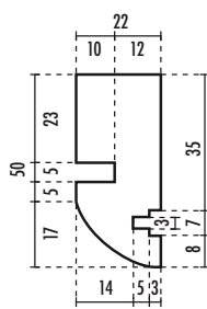
C profilo architrave
