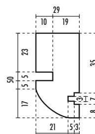
C profilo architrave
